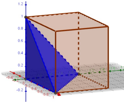
Figure 5.2: Three numbers sum to less than 1.
