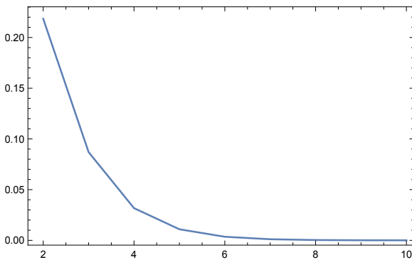
Figure 5.34: Dart throwing in polar coordinates. The bigger the dimension, the less the chance of hitting the center.
