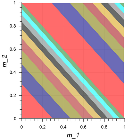
Figure 5.17: Probability of first digit in product, logarithmic scale.
