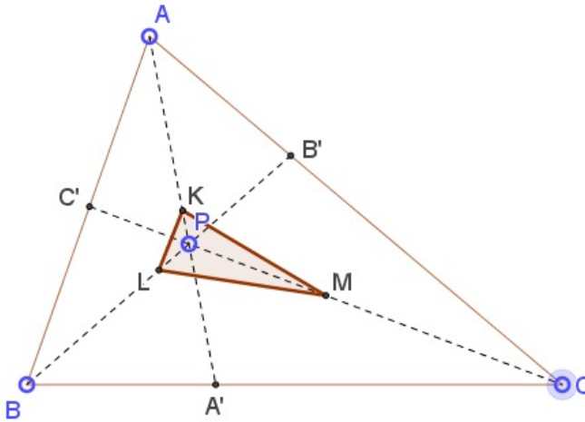
Figure 5.1: Probability in triangle.
