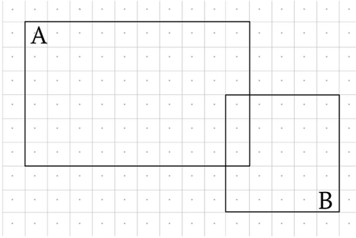
Figure A.1: Dependence depends on sample space.
