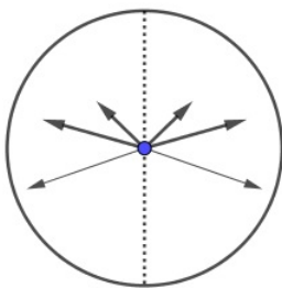
Figure 5.22: Lucky times at a Moscow math olympiad 1.
