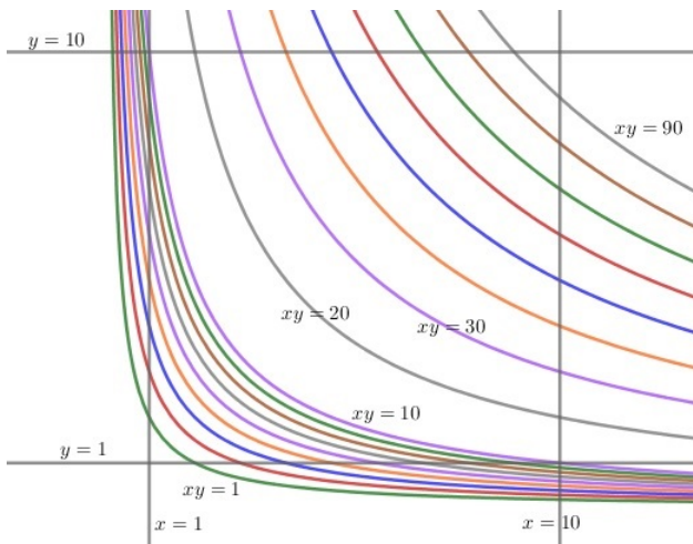
Figure 5.16: Probability of first digit in product.
