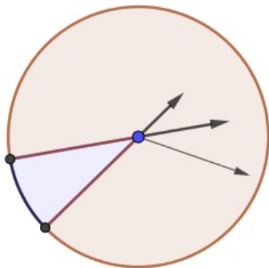
Figure 5.23: Lucky times at a Moscow math olympiad 2.
