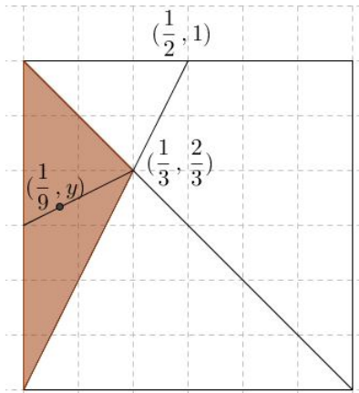
Figure 5.14: Random points on a segment 1.
