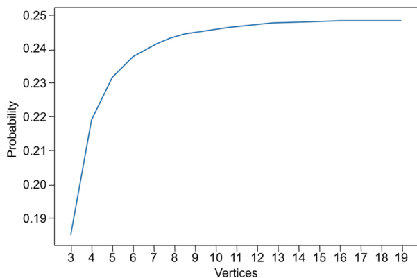
Figure 5.33: Dart throwing in polar coordinates, n -gon board.
