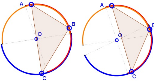
Figure 5.5: A triangle inscribed in a circle may or may not include the center.
