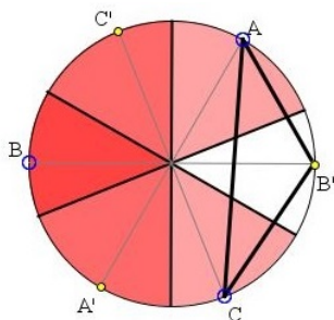
Figure 5.4: How to find an obtuse triangle.
