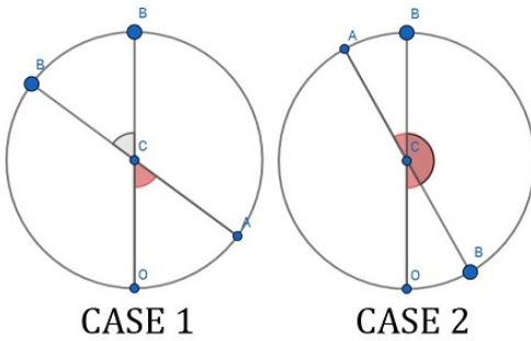
Figure 5.7: Two random points on a circle.
