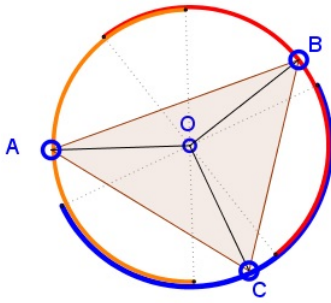
Figure 5.6: Three semicircles that completely cover the circle.
