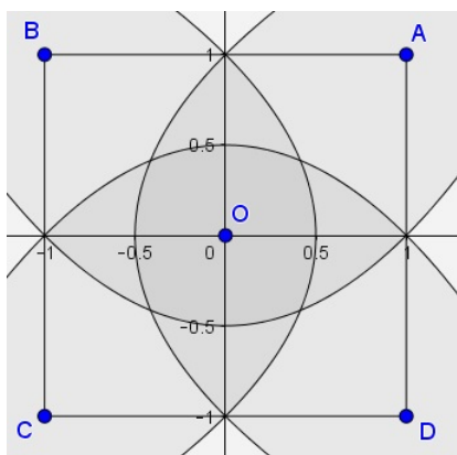
Figure 5.29: Dart throwing: the whole picture.
