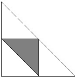
Figure 5.3: A region that yields an acute triangle.
