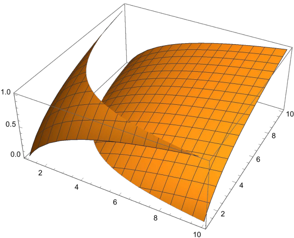
Figure 5.19: Sum of two logarithms 2.
