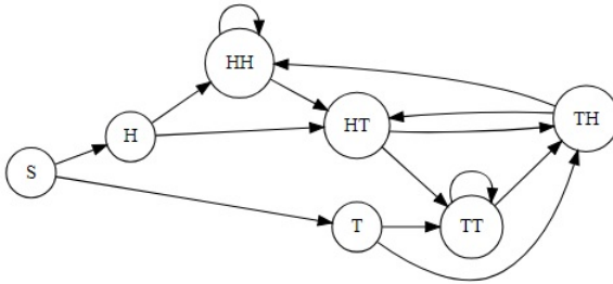
Figure 3.3: Coin tossing: whole picture.
