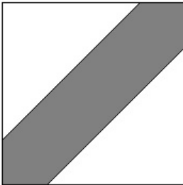
Figure 5.8: Two friends meeting.
