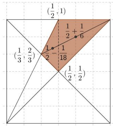
Figure 5.15: Random points on a segment 2.
