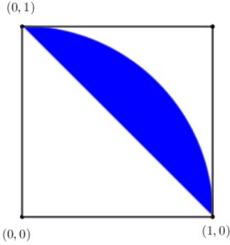
Figure 5.12: Random numbers and obtuse triangle.
