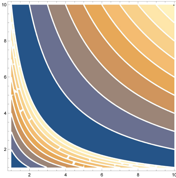
Figure 5.21: Sum of two logarithms: contour plot.
