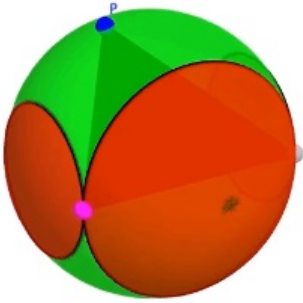
Figure 5.11: Flat probabilities on a sphere: a 3D view.
