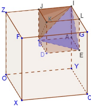
Figure 5.28: Splitting probabilities for one short and two long pieces.
