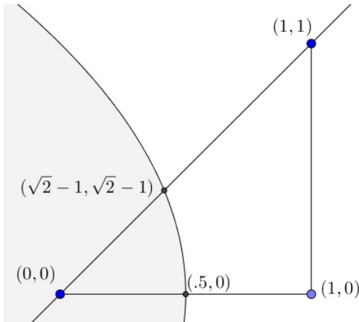
Figure 5.31: Dart throwing: one octant.
