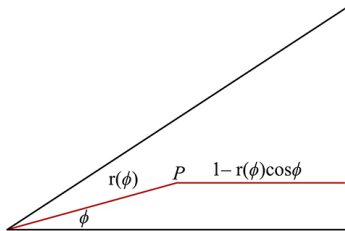
Figure 5.32: Dart throwing in polar coordinates.
