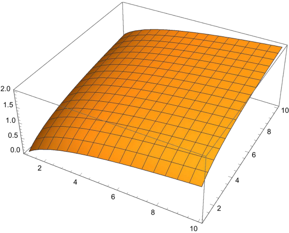
Figure 5.18: Sum of two logarithms 1.
