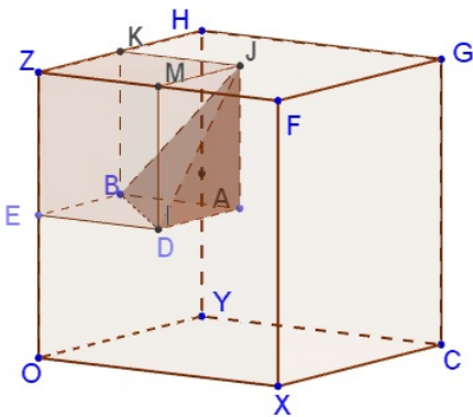
Figure 5.27: Splitting probabilities for two short and one long pieces.
