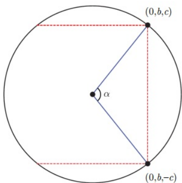
Figure 5.10: A 2D cross section.
